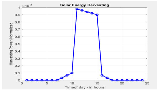
Figure 1. Simulation of a sensor node solar energy harvest process throughout the duration of a 24-hour day
