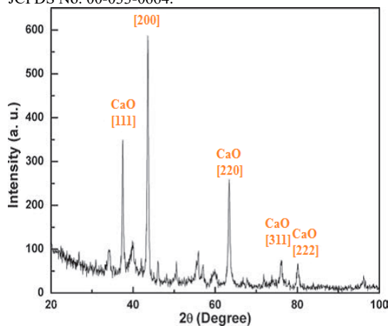
Figure 4: X-ray diffractions of CaO NPs powders after calcination at 900 °C temperatures
