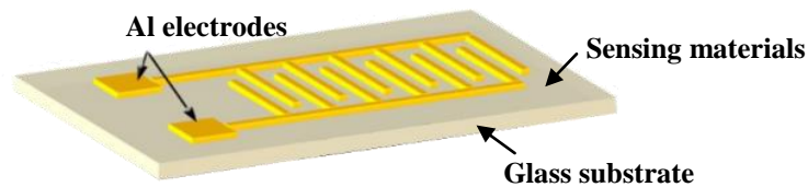
Fig. 3 A schematic of the patterned aluminum electrodes
