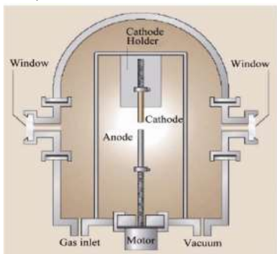
Fig.3: Arc-discharge method to produce SWCNT with aid of catalyst and MWCNT without the catalyst[12]
