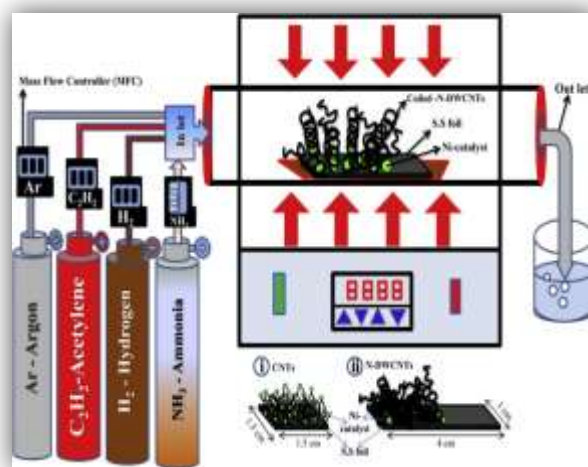
Fig.4:CVD method to produce MWCNT[15].
