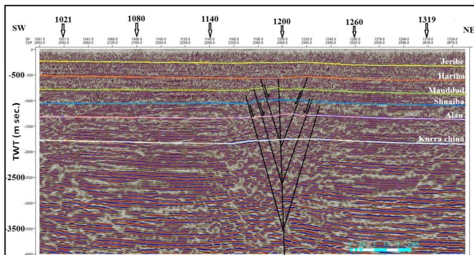
Figure (4) Seismic reflection section WT-36 in Al-Thirthar valley.
