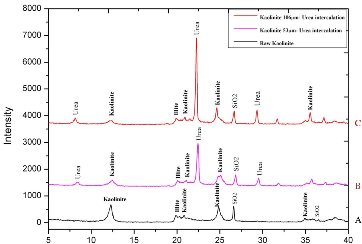
Figure 4: The XRD pattern of raw kaolinite (A), kaolinite 53µm- urea intercalation (B) and kaolinite 106µm- urea intercalation (C)
