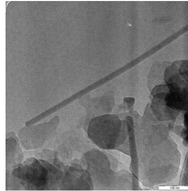
Figure 6. TEM image of Kaolinite 106µm Urea complexes
