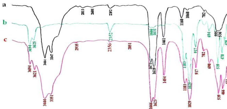
Figure 2: FTIR spectra of (A) kaolin 106 \mu\text{m} , (B) Urea and (C) Kaolin 106 \mu\text{m} - urea complex
