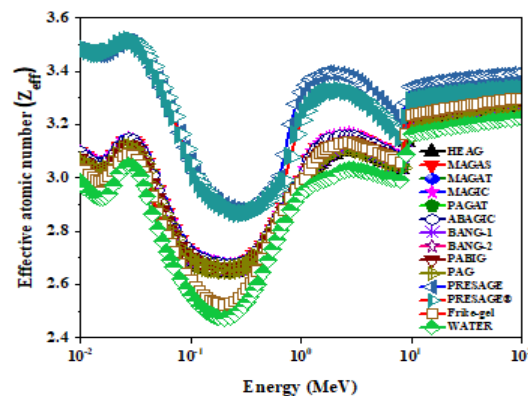
Fig. 1. Variation of effective atomic number Z_{\text{eff}} of dosimetric gels with the kinetic energy of He ion.
