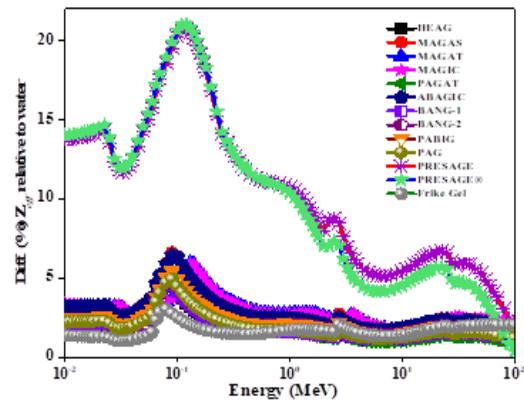
Fig. 15. Percentage difference in Z_{\text{eff}} of gel dosimeters relative to water for C ion interaction.
