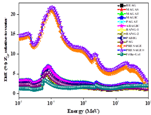
Fig. 14. Percentage difference in Z_{\text{eff}} of gel dosimeters relative to water for B ion interaction.
