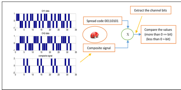
Figure 6 Cdma Receiver.
