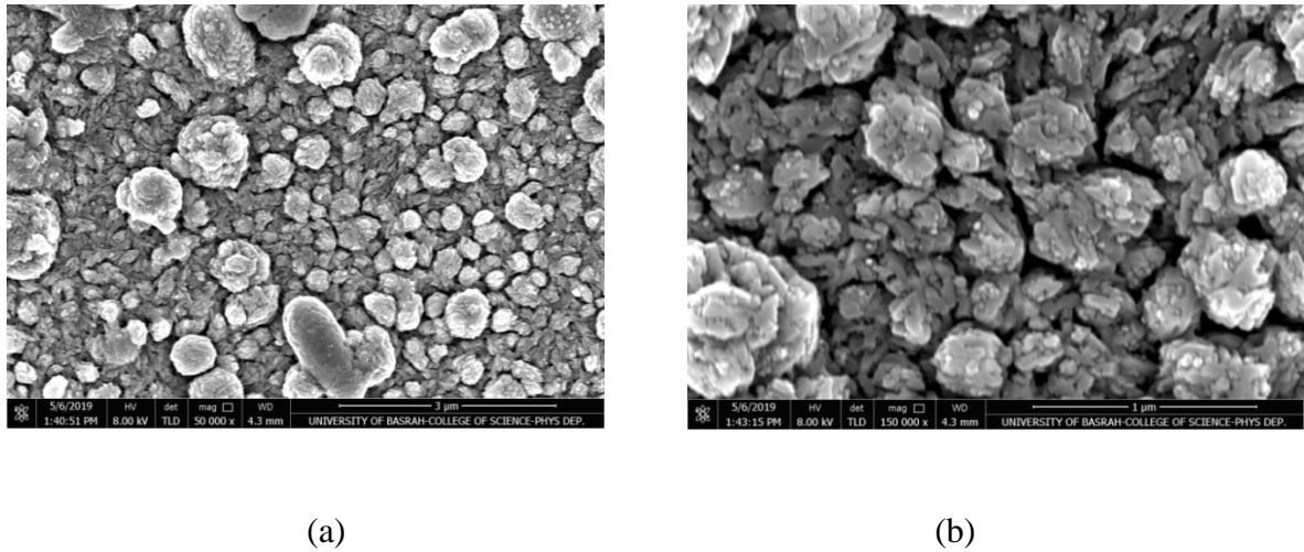
Fig.3: (a, b) Topographic composition and average size of the prepared laser pulse nanoparticles (500 pulse).
