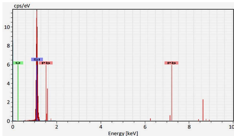
Fig.4: EDX spectrum analysis of lead nanoparticles.
