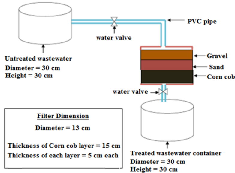
Figure 2. Illustration of the filter B
