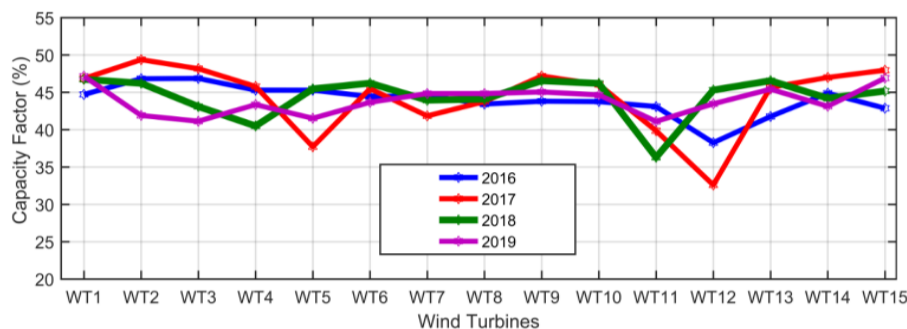
Figure 7. Capacity factor 2016-2019
