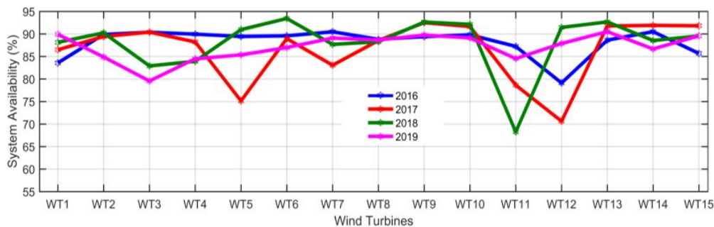
Figure 6. System availability 2016-2019
