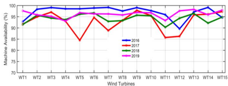
Figure 4. Machine availability
