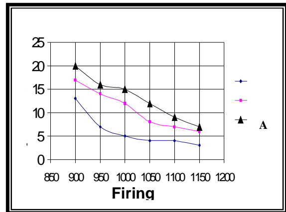
Fig(2) Apparent porosity of different mixes
