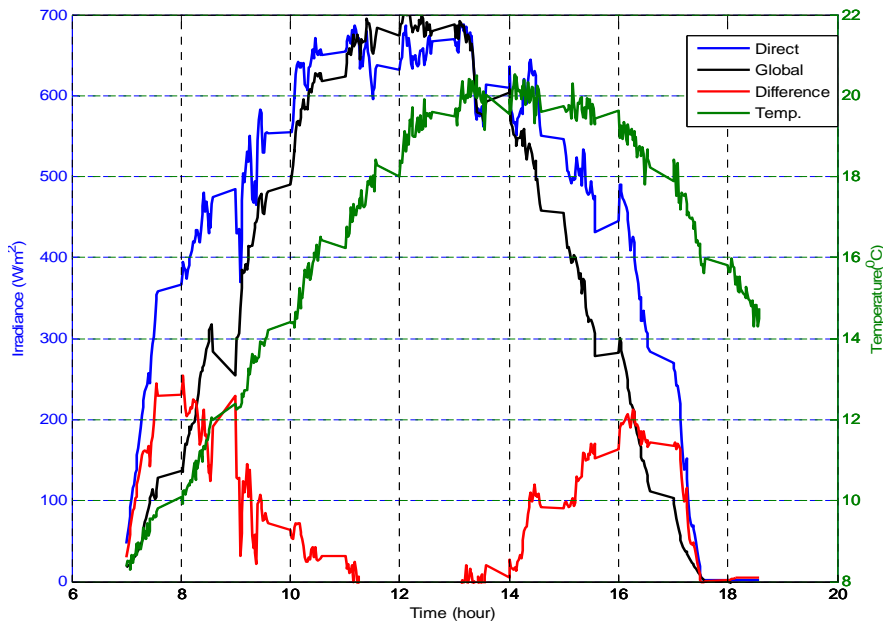
Figure 1. Average monthly irradiance for January-2013 (the average for each two minutes)
