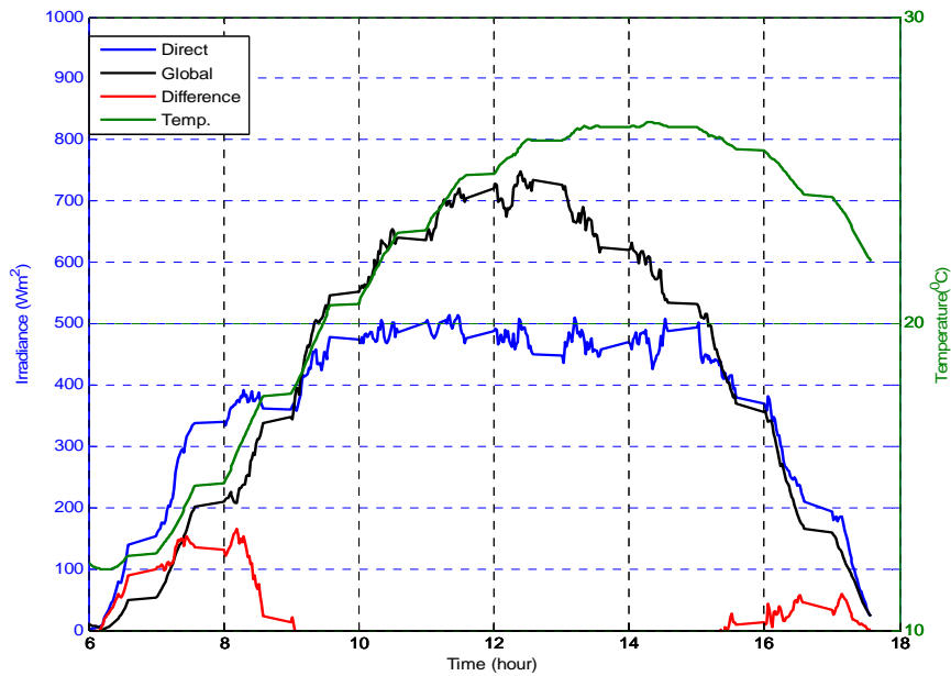
Figure 5. Average monthly irradiance for March-2013 (the average for each two minutes)
