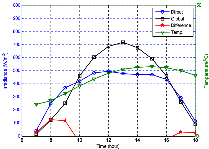
Figure 6. Hourly average irradiance for March-2013
