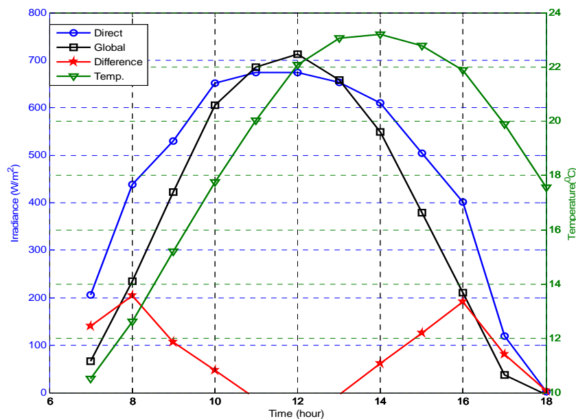
Figure 4. Hourly average irradiance for February-2013
