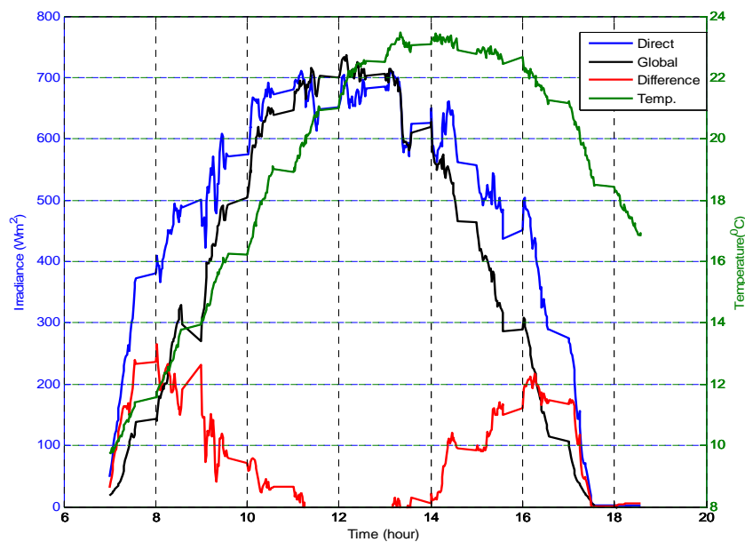
Figure 3. Average monthly irradiance for February-2013 (the average for each two minutes)
