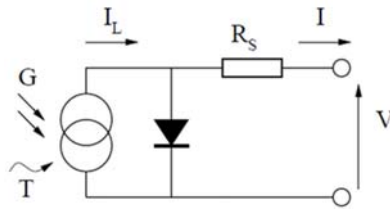
Figure 1. Solar cell with single-diode and series resistance
